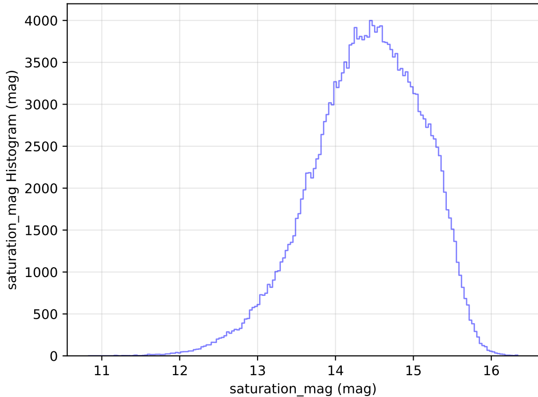
too_elab_heavy_r128_d2_gz_v3.4_10yrs All sky g band: saturation_mag Histogram
