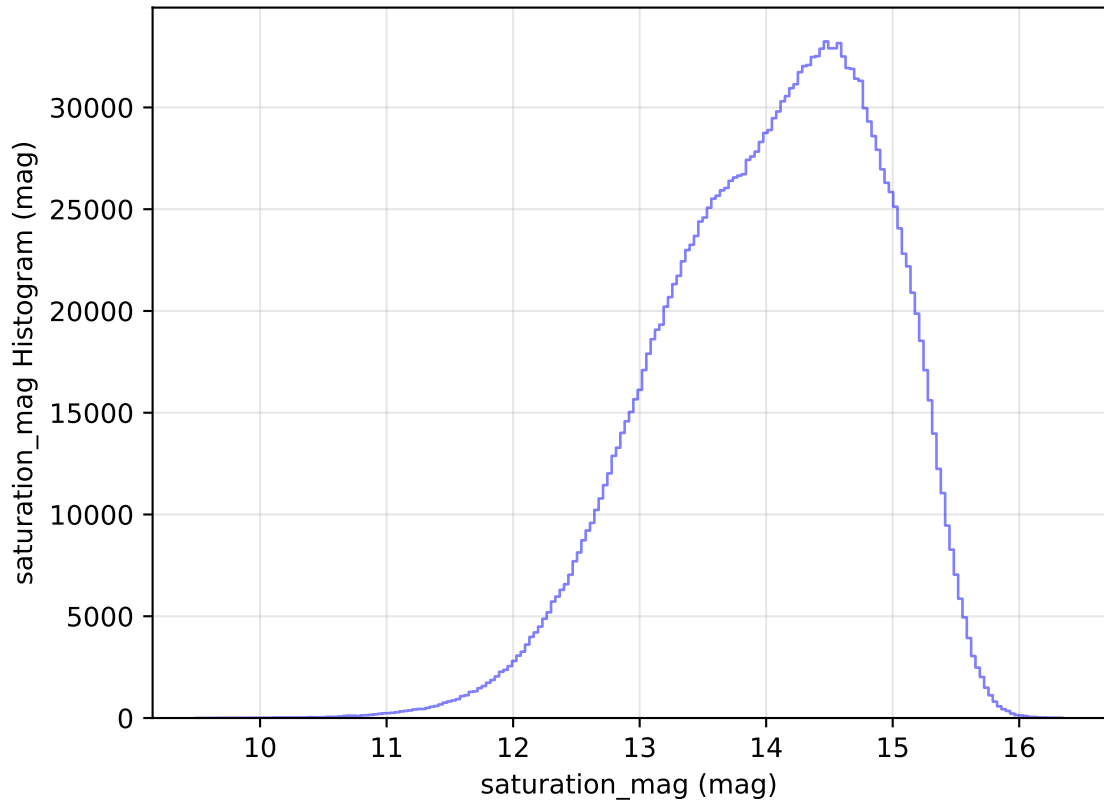
too_elab_heavy_r128_d2_gz_v3.4_10yrs All sky all bands: saturation_mag Histogram
