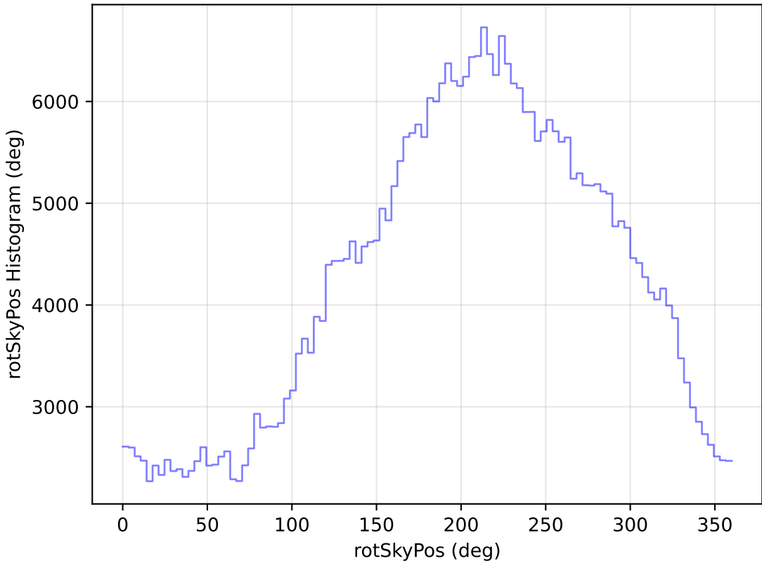
too_elab_heavy_r128_d2_gz_v3.4_10yrs WFD z band: rotSkyPos Histogram
