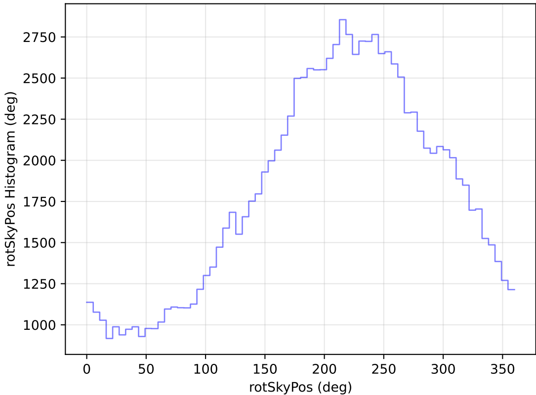
too_elab_heavy_r128_d2_gz_v3.4_10yrs WFD u band: rotSkyPos Histogram
