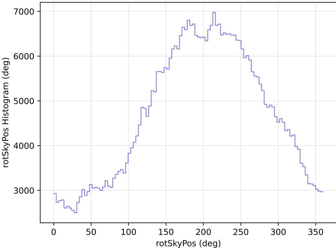
too_elab_heavy_r128_d2_gz_v3.4_10yrs WFD r band: rotSkyPos Histogram
