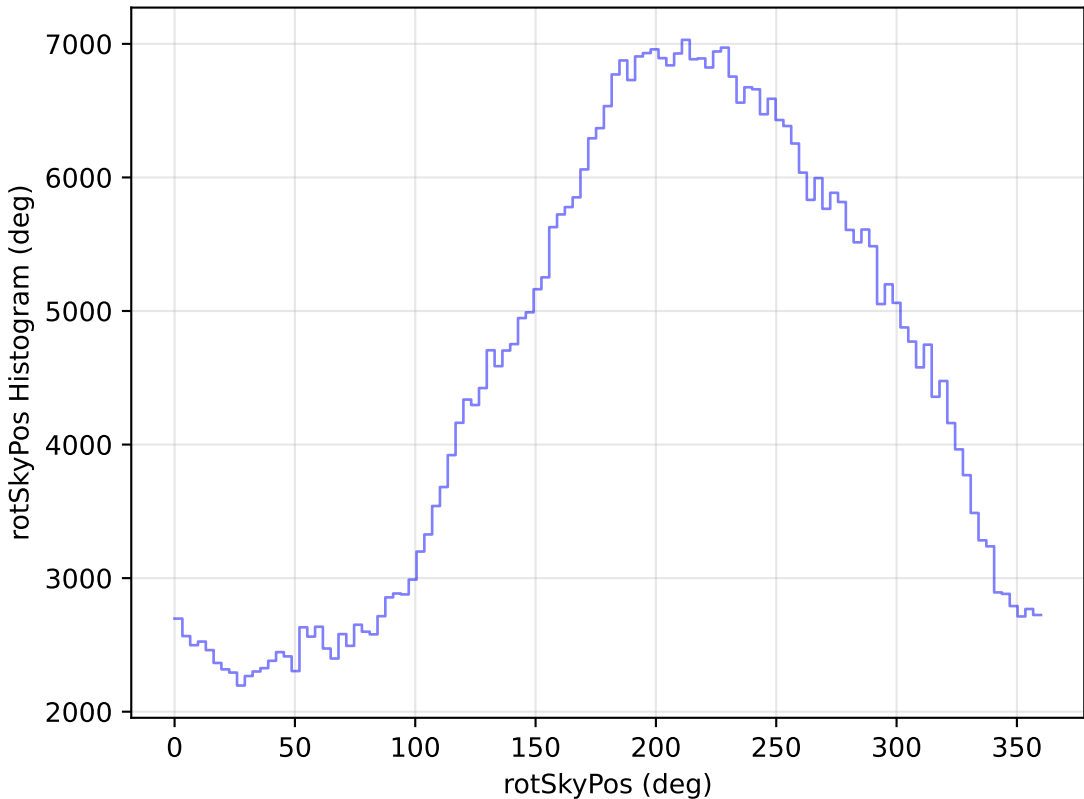
too_elab_heavy_r128_d2_gz_v3.4_10yrs WFD i band: rotSkyPos Histogram
