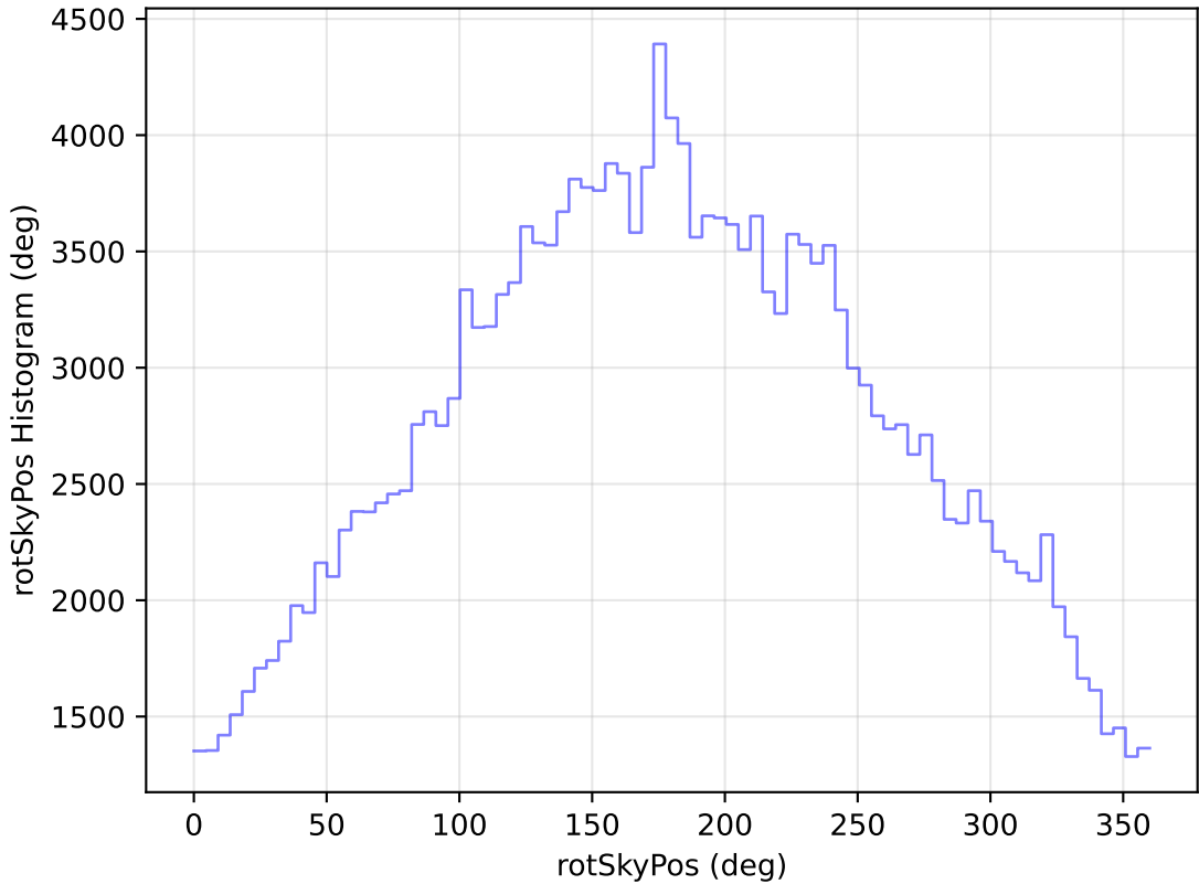
too_elab_heavy_r128_d2_gz_v3.4_10yrs WFD g band: rotSkyPos Histogram
