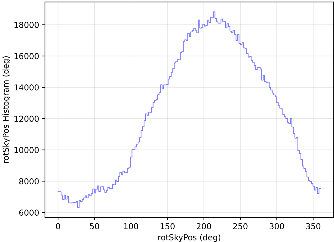
too_elab_heavy_r128_d2_gz_v3.4_10yrs WFD all bands: rotSkyPos Histogram
