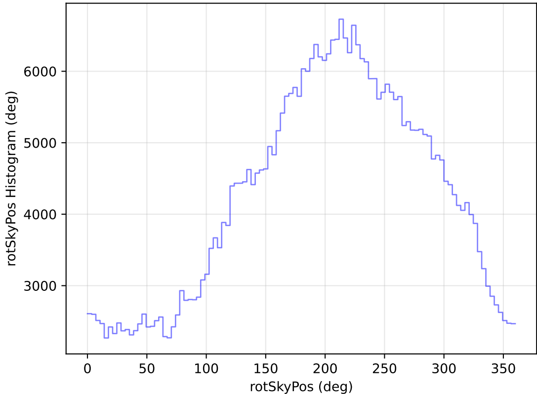
too_elab_heavy_r128_d2_gz_v3.4_10yrs All sky z band: rotSkyPos Histogram
