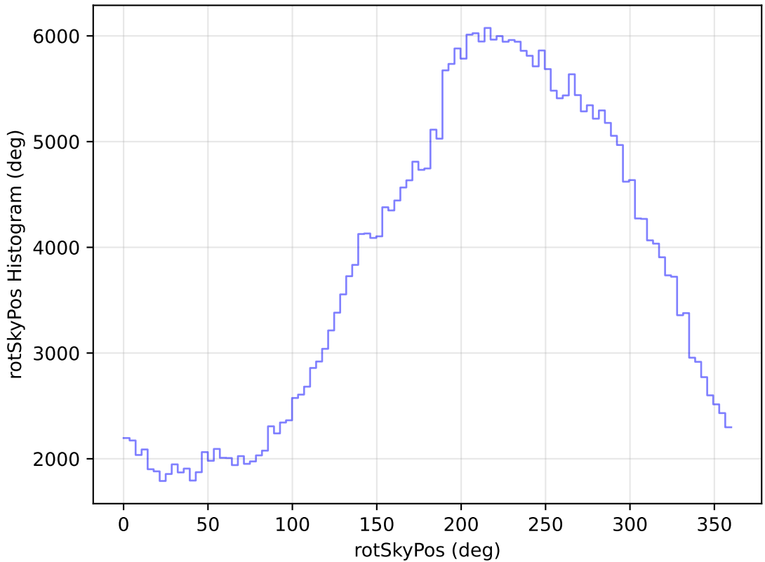
too_elab_heavy_r128_d2_gz_v3.4_10yrs All sky y band: rotSkyPos Histogram
