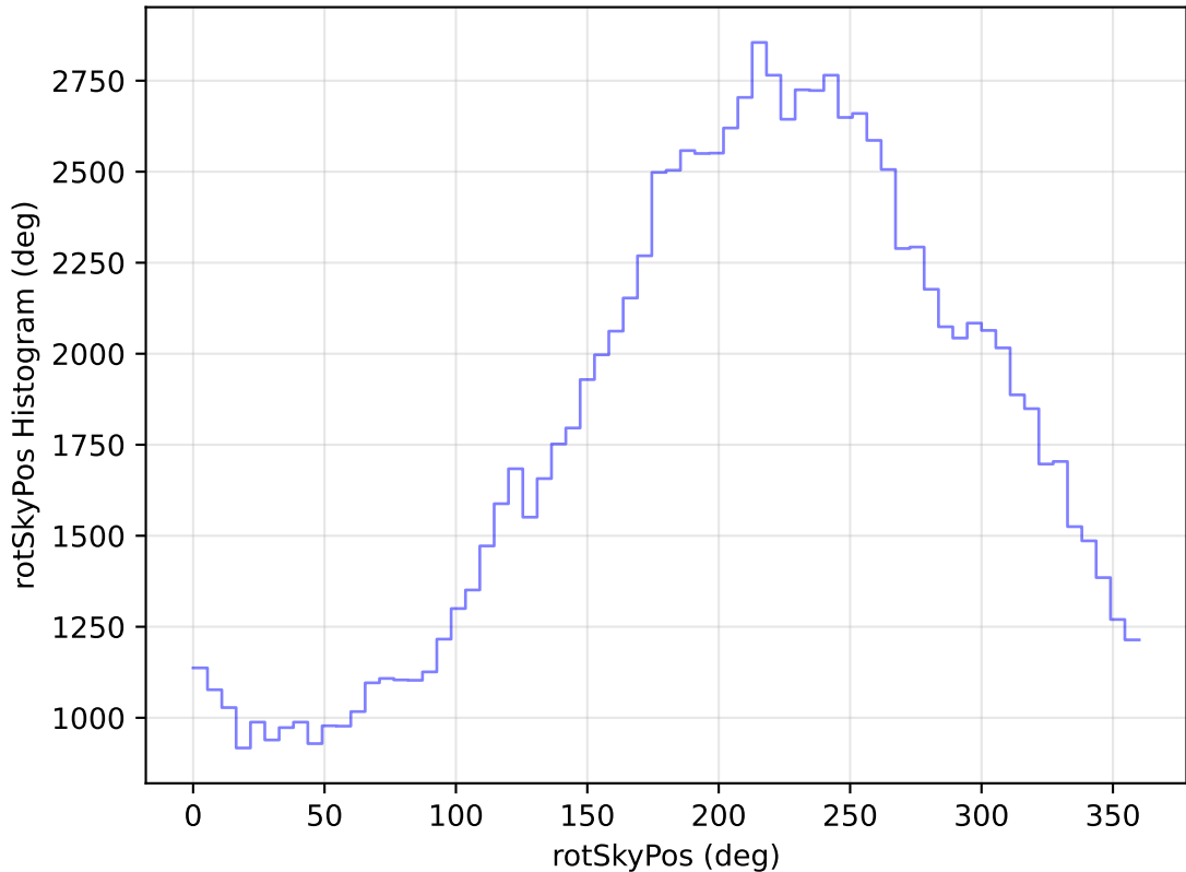
too_elab_heavy_r128_d2_gz_v3.4_10yrs All sky u band: rotSkyPos Histogram
