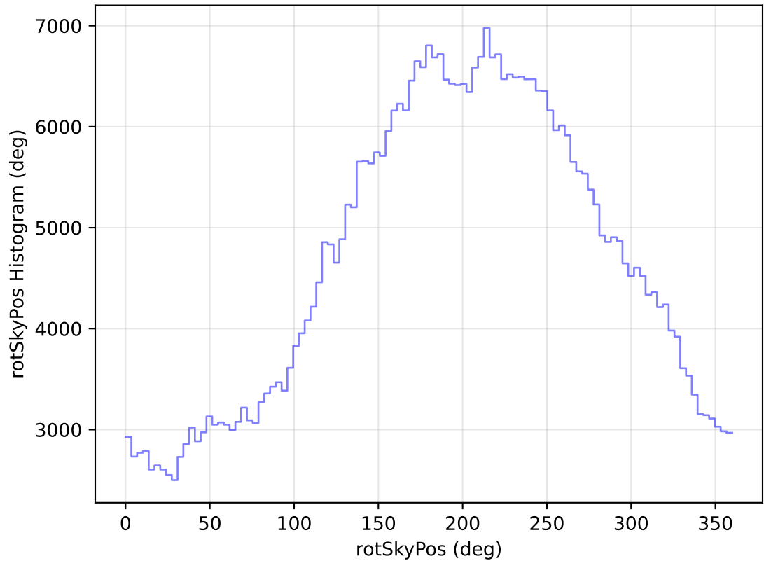
too_elab_heavy_r128_d2_gz_v3.4_10yrs All sky r band: rotSkyPos Histogram
