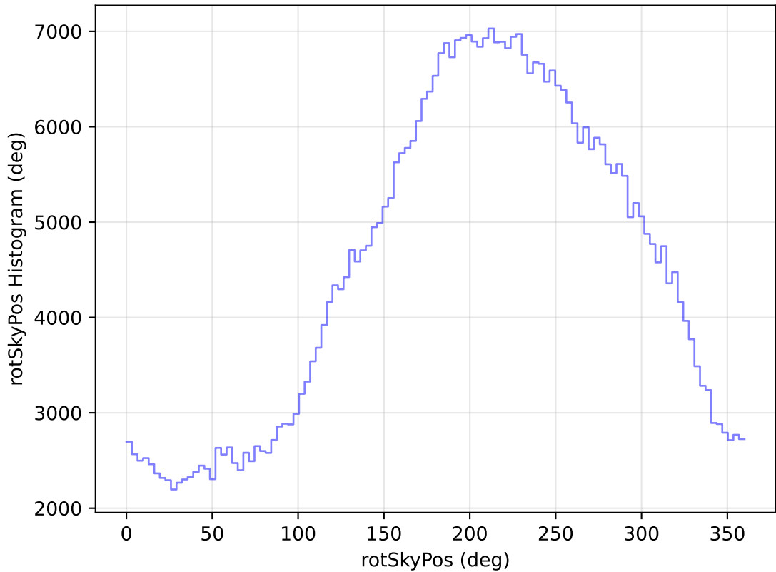
too_elab_heavy_r128_d2_gz_v3.4_10yrs All sky i band: rotSkyPos Histogram
