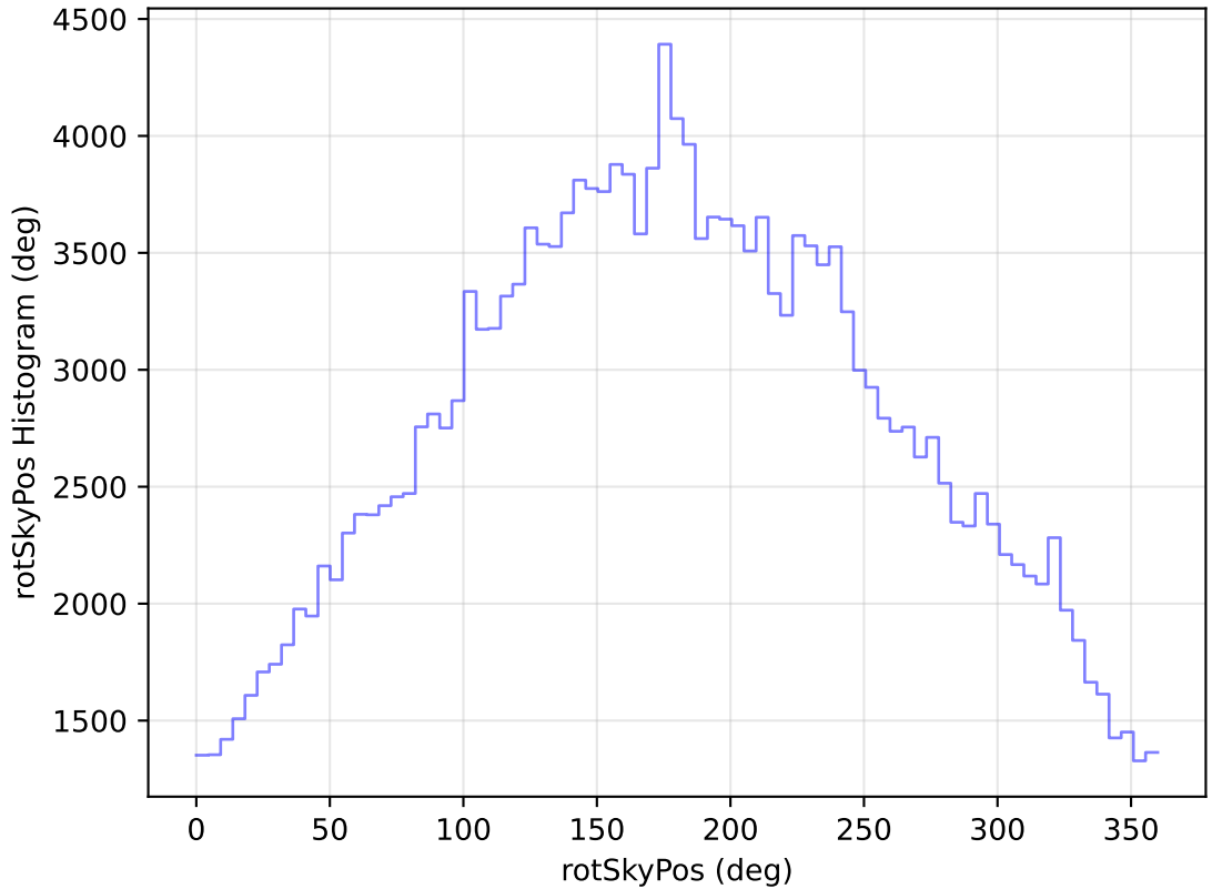
too_elab_heavy_r128_d2_gz_v3.4_10yrs All sky g band: rotSkyPos Histogram
