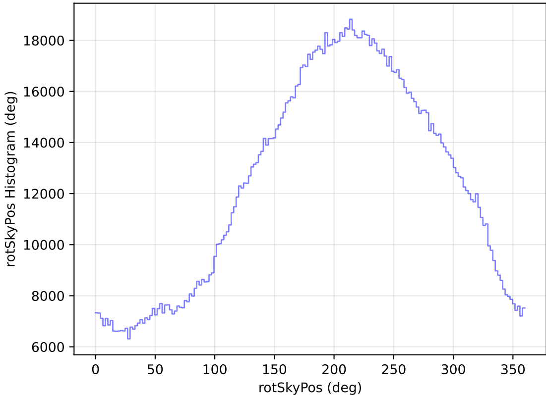
too_elab_heavy_r128_d2_gz_v3.4_10yrs All sky all bands: rotSkyPos Histogram
