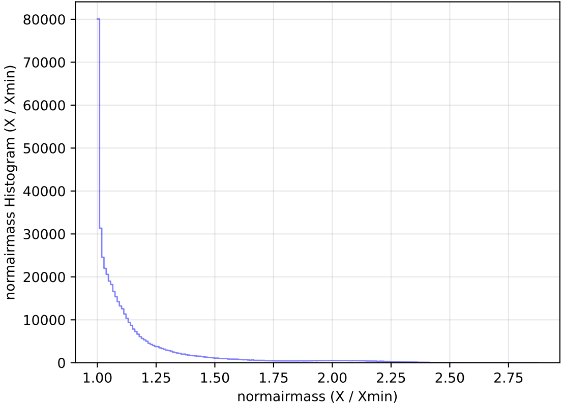
too_elab_heavy_r128_d2_gz_v3.4_10yrs WFD r band: normairmass Histogram
