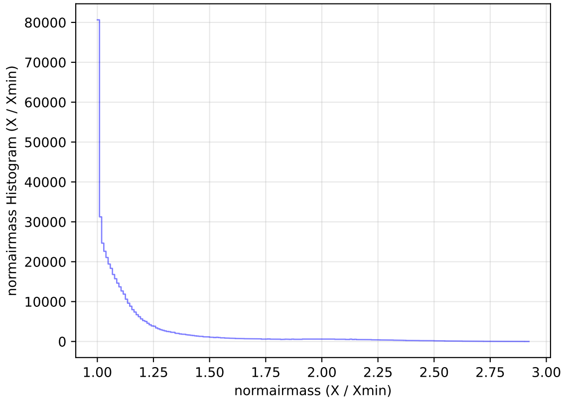
too_elab_heavy_r128_d2_gz_v3.4_10yrs WFD i band: normairmass Histogram
