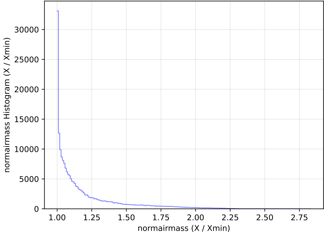
too_elab_heavy_r128_d2_gz_v3.4_10yrs WFD g band: normairmass Histogram
