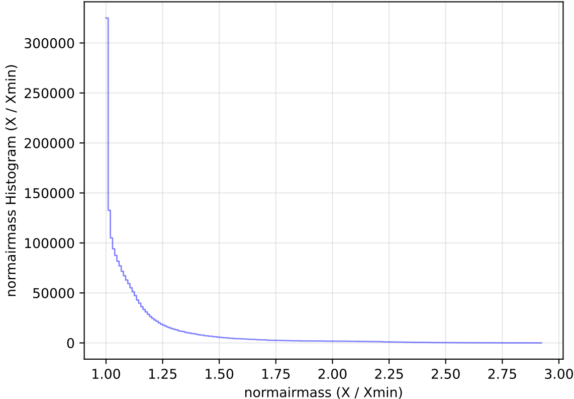
too_elab_heavy_r128_d2_gz_v3.4_10yrs WFD all bands: normairmass Histogram
