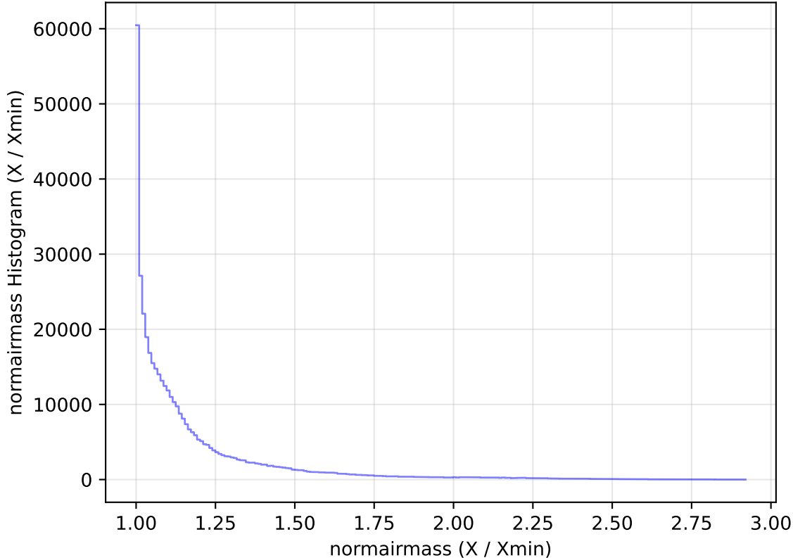
too_elab_heavy_r128_d2_gz_v3.4_10yrs All sky z band: normairmass Histogram
