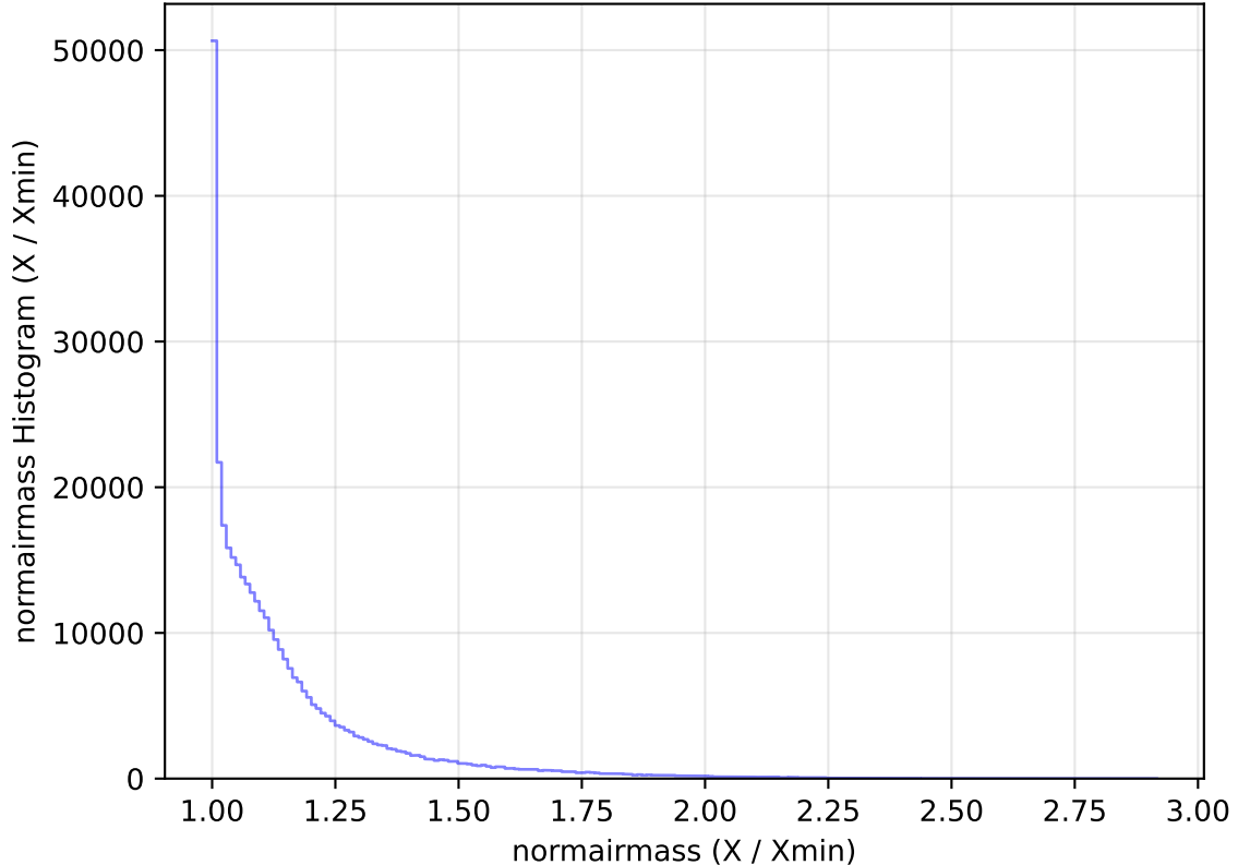
too_elab_heavy_r128_d2_gz_v3.4_10yrs All sky y band: normairmass Histogram
