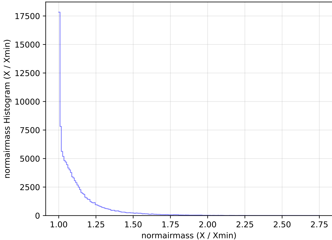
too_elab_heavy_r128_d2_gz_v3.4_10yrs All sky u band: normairmass Histogram
