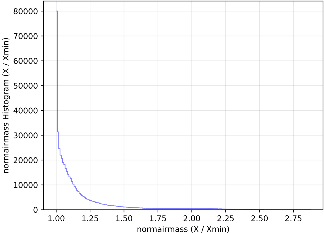
too_elab_heavy_r128_d2_gz_v3.4_10yrs All sky r band: normairmass Histogram
