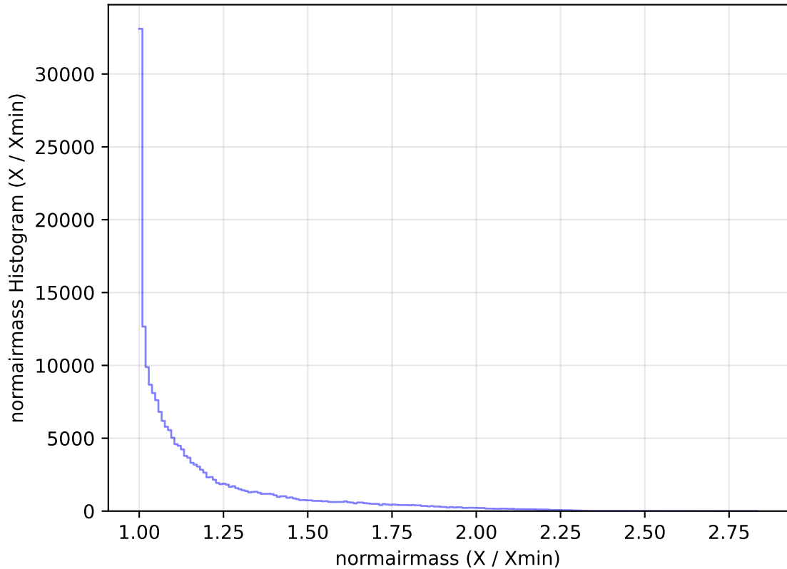
too_elab_heavy_r128_d2_gz_v3.4_10yrs All sky g band: normairmass Histogram
