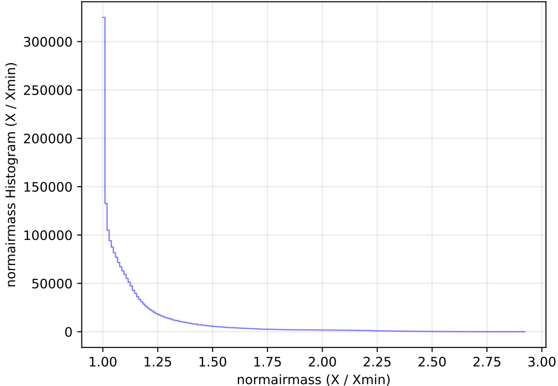
too_elab_heavy_r128_d2_gz_v3.4_10yrs All sky all bands: normairmass Histogram
