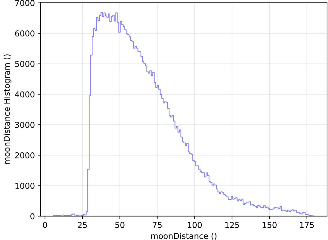
too_elab_heavy_r128_d2_gz_v3.4_10yrs WFD y band: moonDistance Histogram
