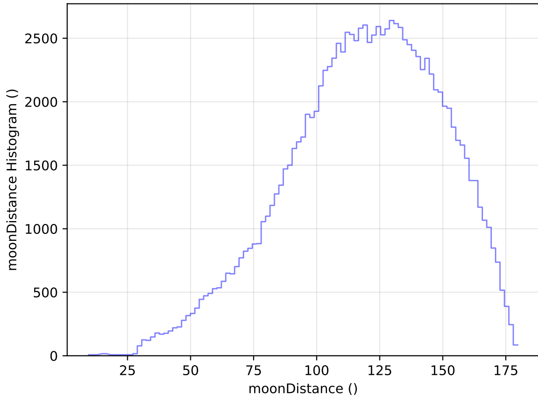
too_elab_heavy_r128_d2_gz_v3.4_10yrs WFD u band: moonDistance Histogram
