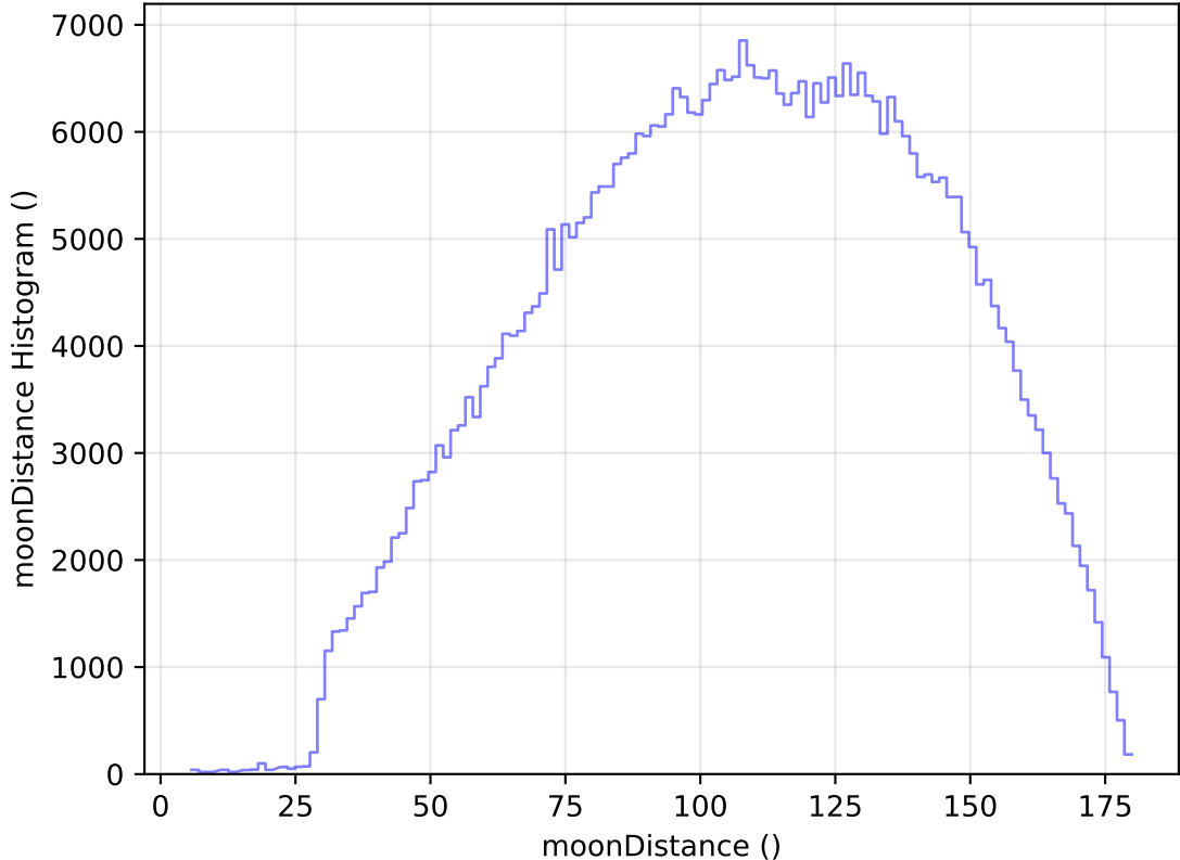
too_elab_heavy_r128_d2_gz_v3.4_10yrs WFD r band: moonDistance Histogram
