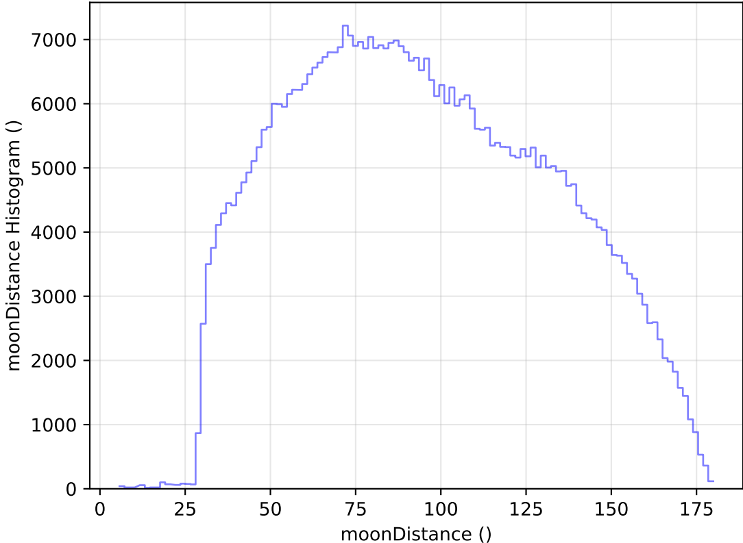
too_elab_heavy_r128_d2_gz_v3.4_10yrs WFD i band: moonDistance Histogram
