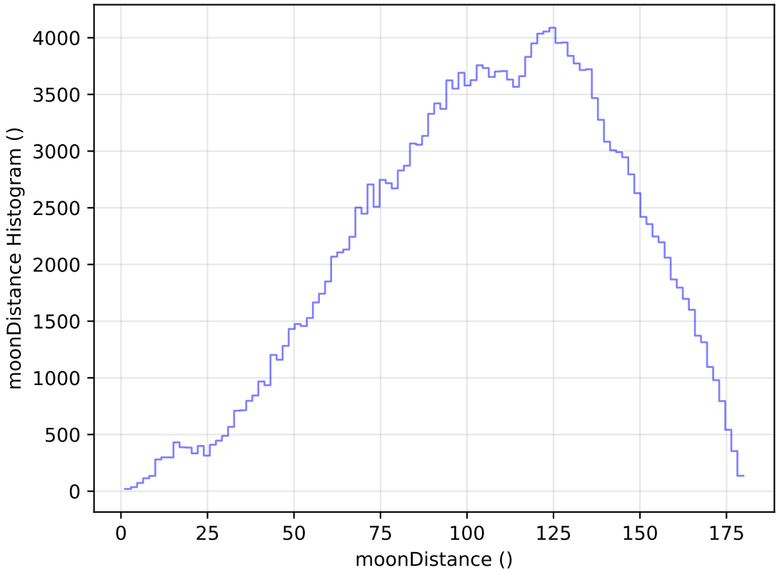
too_elab_heavy_r128_d2_gz_v3.4_10yrs WFD g band: moonDistance Histogram
