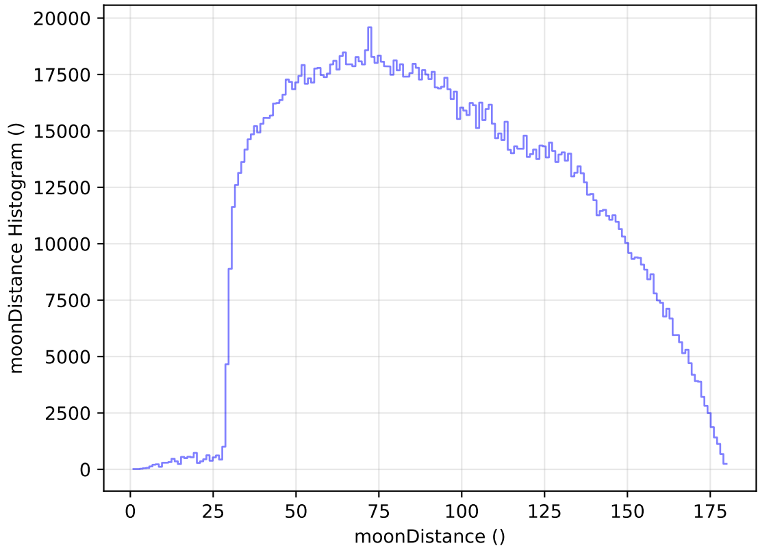
too_elab_heavy_r128_d2_gz_v3.4_10yrs WFD all bands: moonDistance Histogram
