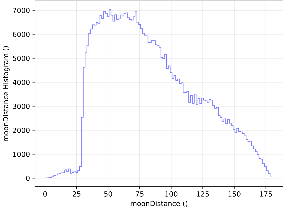
too_elab_heavy_r128_d2_gz_v3.4_10yrs All sky z band: moonDistance Histogram
