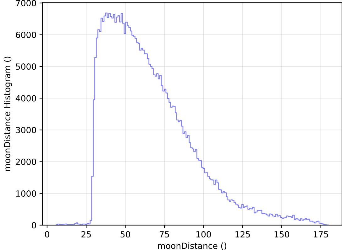
too_elab_heavy_r128_d2_gz_v3.4_10yrs All sky y band: moonDistance Histogram
