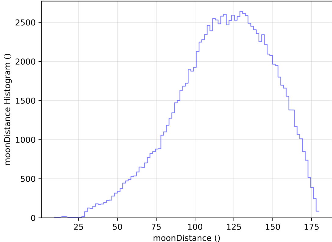
too_elab_heavy_r128_d2_gz_v3.4_10yrs All sky u band: moonDistance Histogram
