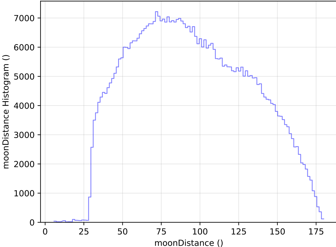
too_elab_heavy_r128_d2_gz_v3.4_10yrs All sky i band: moonDistance Histogram
