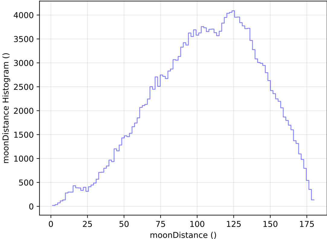
too_elab_heavy_r128_d2_gz_v3.4_10yrs All sky g band: moonDistance Histogram
