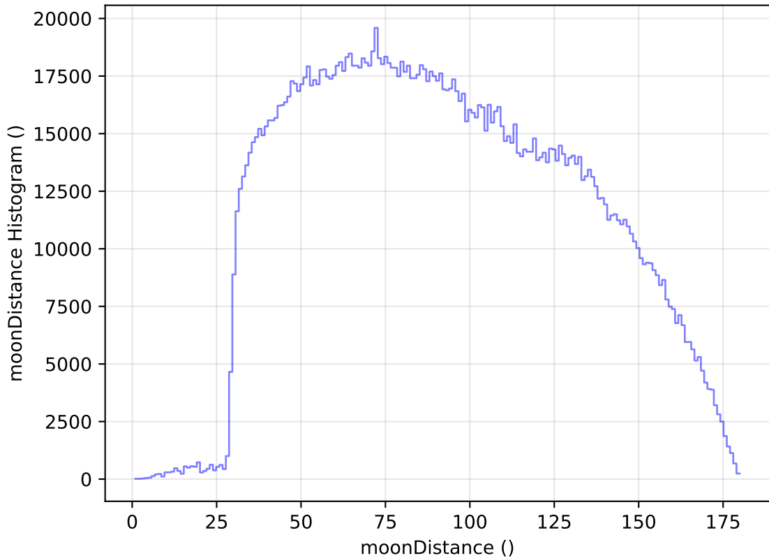
too_elab_heavy_r128_d2_gz_v3.4_10yrs All sky all bands: moonDistance Histogram
