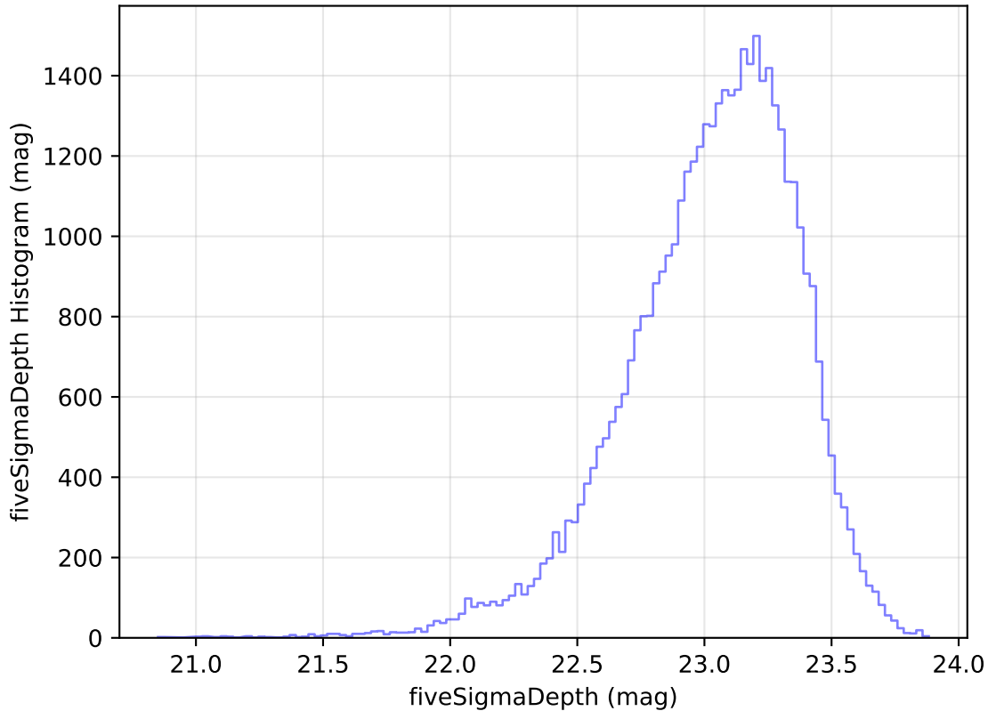
too_elab_heavy_r128_d2_gz_v3.4_10yrs Yr 1 z band: fiveSigmaDepth Histogram
