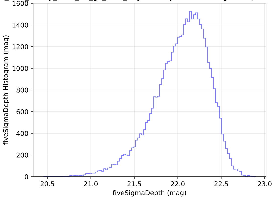
too_elab_heavy_r128_d2_gz_v3.4_10yrs Yr 1 y band: fiveSigmaDepth Histogram
