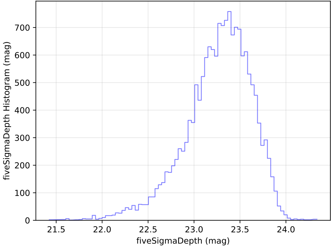
too_elab_heavy_r128_d2_gz_v3.4_10yrs Yr 1 u band: fiveSigmaDepth Histogram
