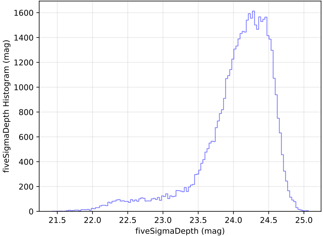
too_elab_heavy_r128_d2_gz_v3.4_10yrs Yr 1 r band: fiveSigmaDepth Histogram
