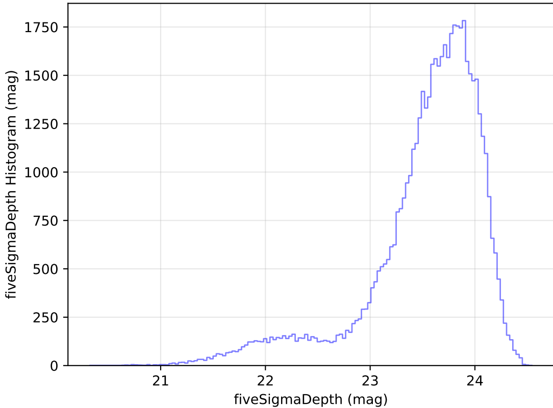
too_elab_heavy_r128_d2_gz_v3.4_10yrs Yr 1 i band: fiveSigmaDepth Histogram
