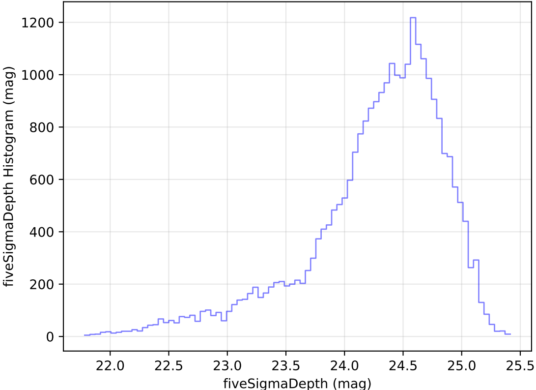
too_elab_heavy_r128_d2_gz_v3.4_10yrs Yr 1 g band: fiveSigmaDepth Histogram
