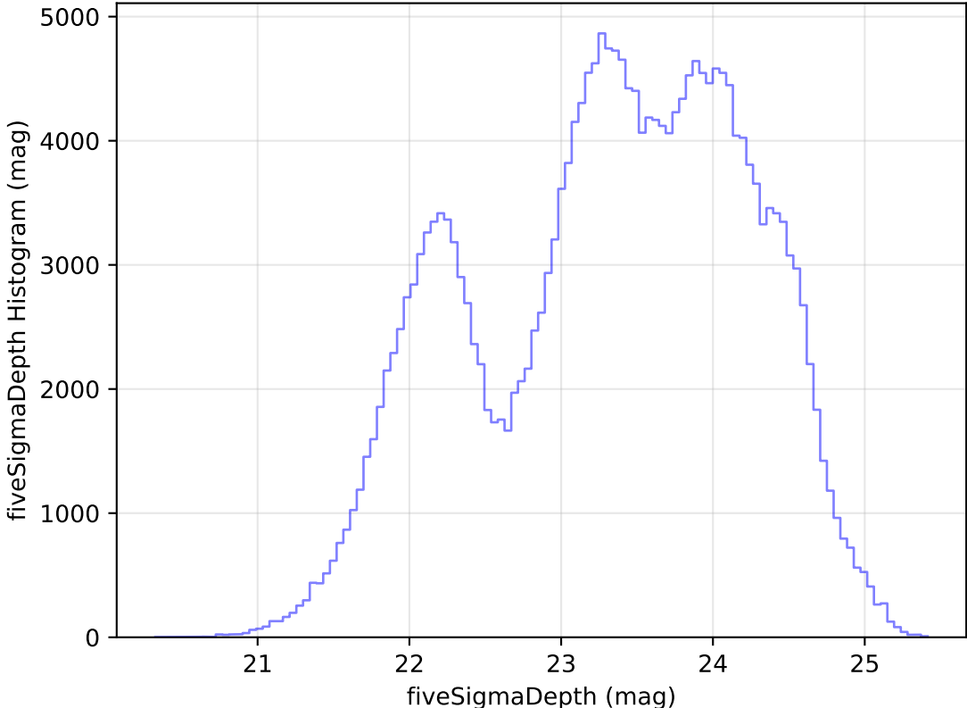
too_elab_heavy_r128_d2_gz_v3.4_10yrs Yr 1 all bands: fiveSigmaDepth Histogram
