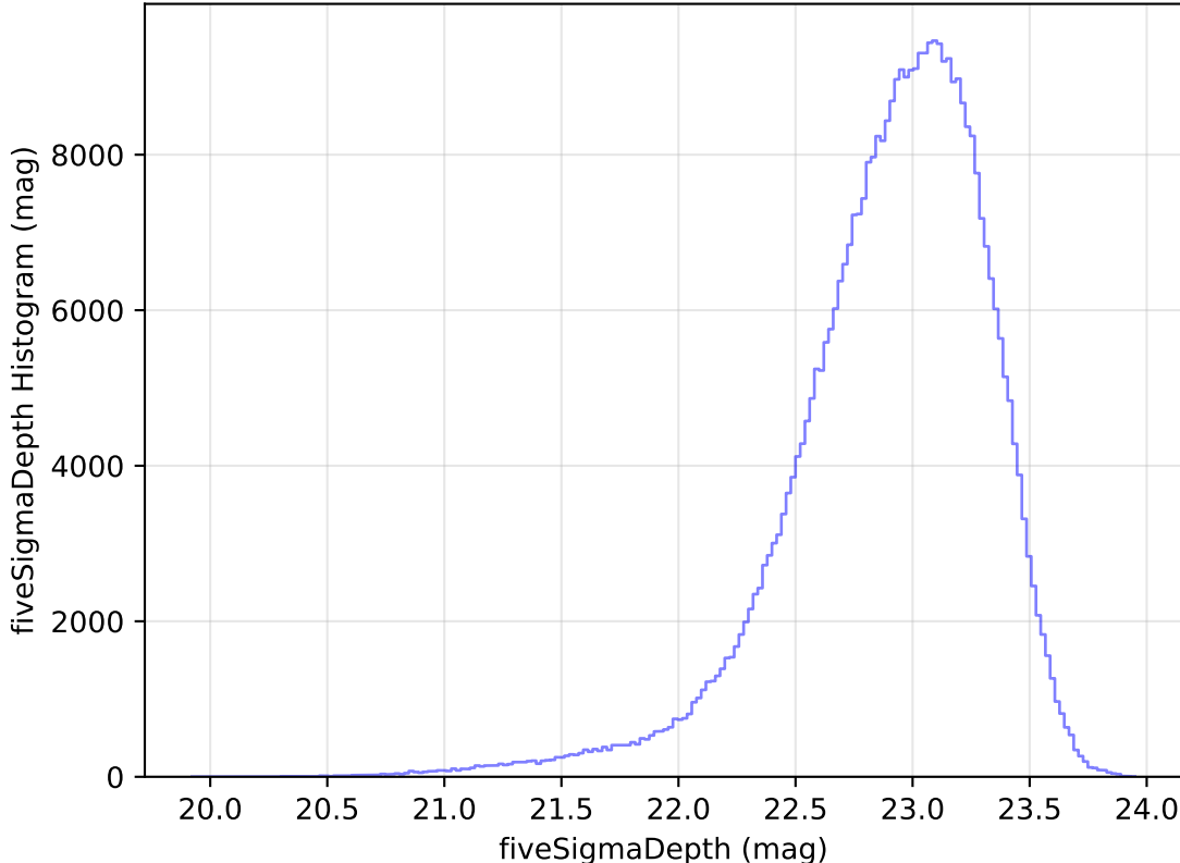
too_elab_heavy_r128_d2_gz_v3.4_10yrs WFD z band: fiveSigmaDepth Histogram
