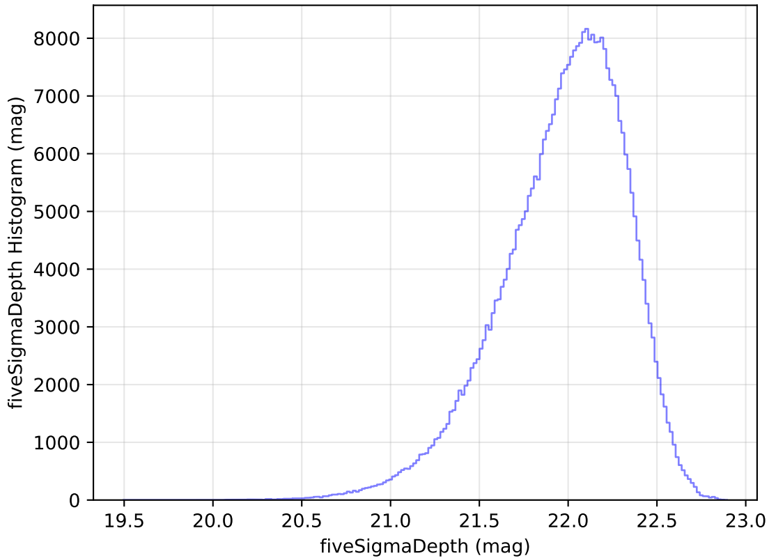
too_elab_heavy_r128_d2_gz_v3.4_10yrs WFD y band: fiveSigmaDepth Histogram
