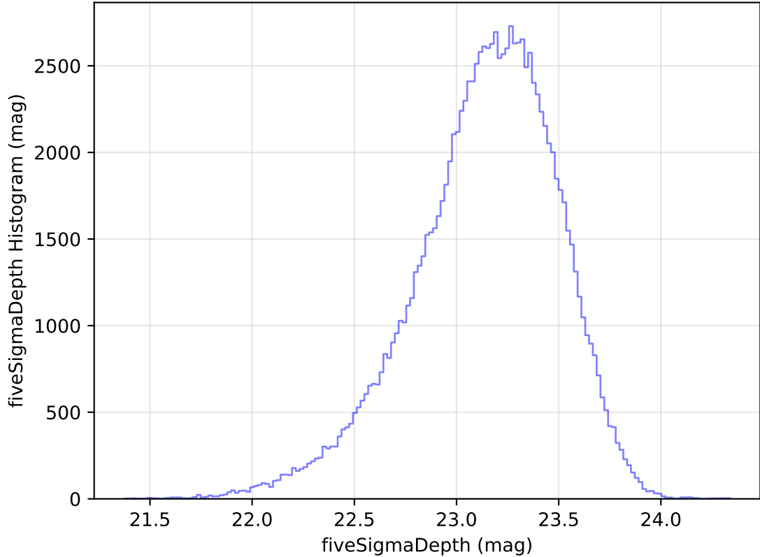
too_elab_heavy_r128_d2_gz_v3.4_10yrs WFD u band: fiveSigmaDepth Histogram
