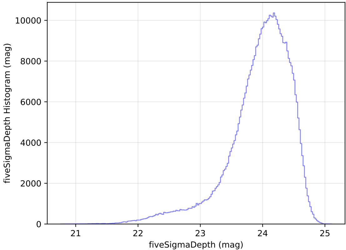
too_elab_heavy_r128_d2_gz_v3.4_10yrs WFD r band: fiveSigmaDepth Histogram
