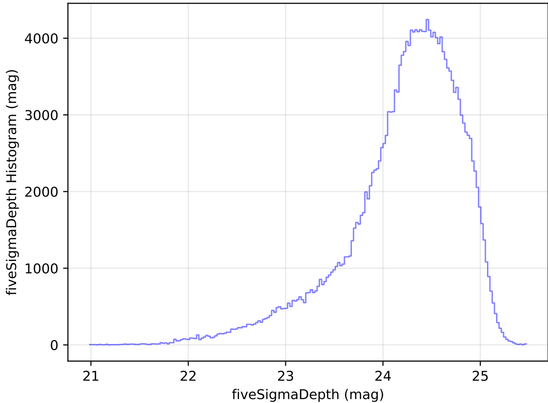
too_elab_heavy_r128_d2_gz_v3.4_10yrs WFD g band: fiveSigmaDepth Histogram
