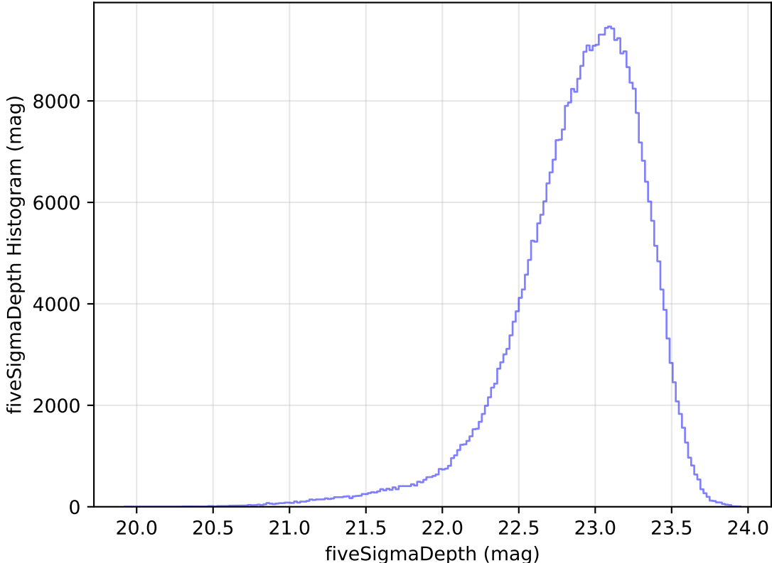
too_elab_heavy_r128_d2_gz_v3.4_10yrs All sky z band: fiveSigmaDepth Histogram
